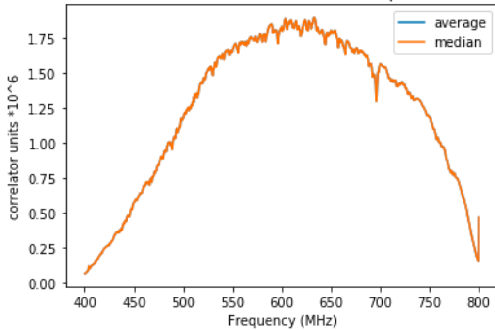
Autocorrelation of 50 ohm terminated x pol west dish
